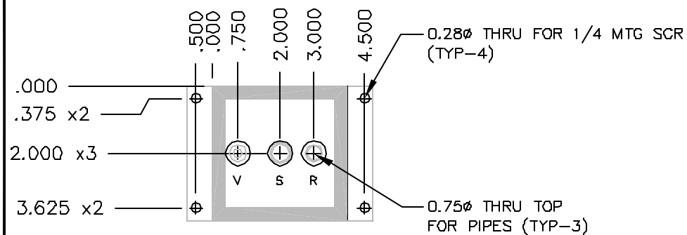
PUMP MTG. TO RESERVOIR DRILL DIMENSIONS
